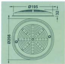
EM2830 – ABS
