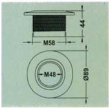
EM2822 – ABS
