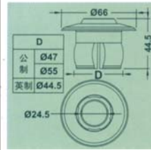
EM33-01 – ABS
