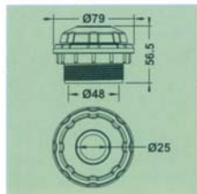
EM233-02 – ABS
